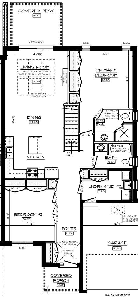
SOUTH BLOCK II - UNIT #5
