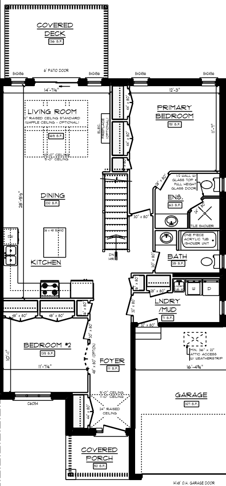
SOUTH BLOCK II - UNIT #3
