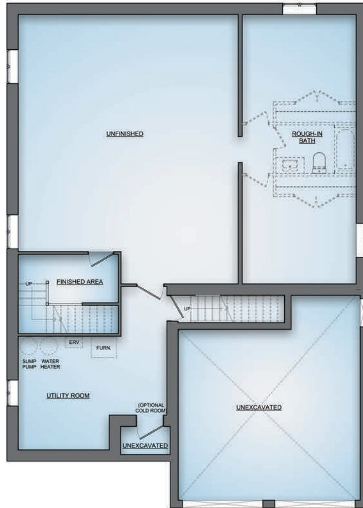
BASEMENT FLOOR
