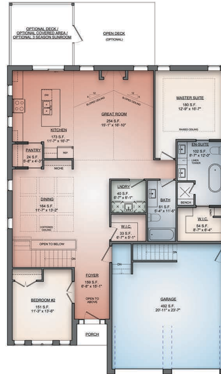
MAIN FLOOR
