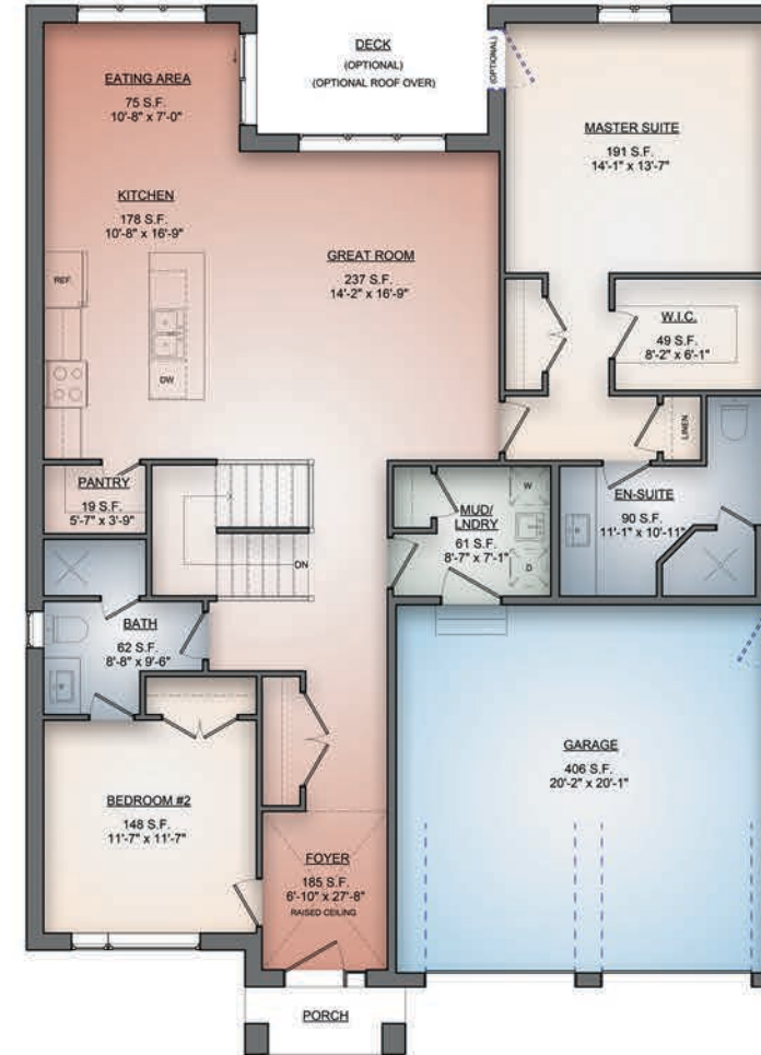
MAIN FLOOR PLAN - ELEVATION A
