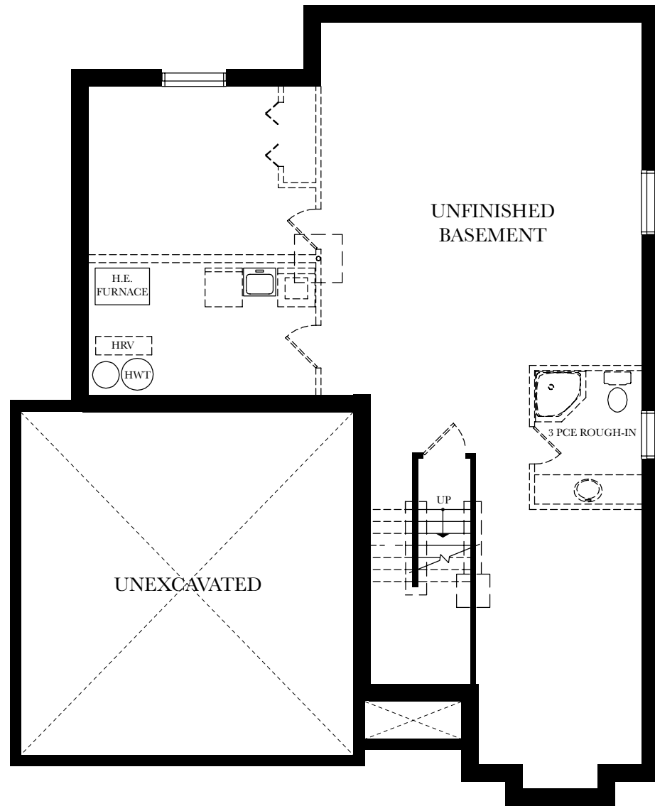
BASEMENT PLAN
