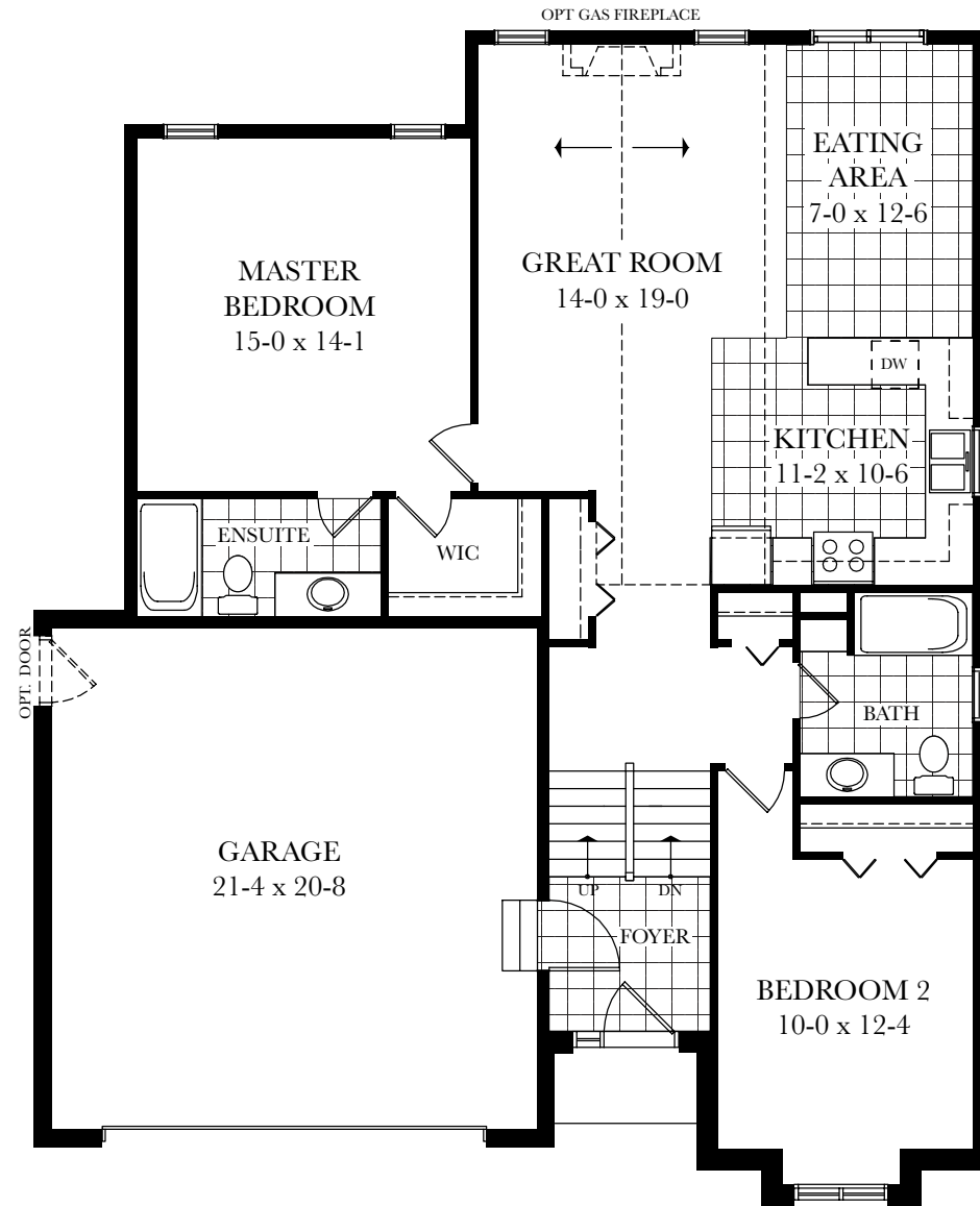
MAIN FLOOR PLAN - 1290 sq.ft.
