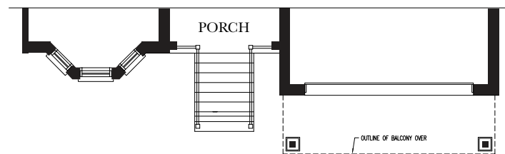
MAIN FLOOR PLAN ELEV. B - 1384 sq.ft
