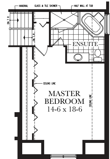
SECOND FLOOR PLAN ELEV. A - 557sq.ft
