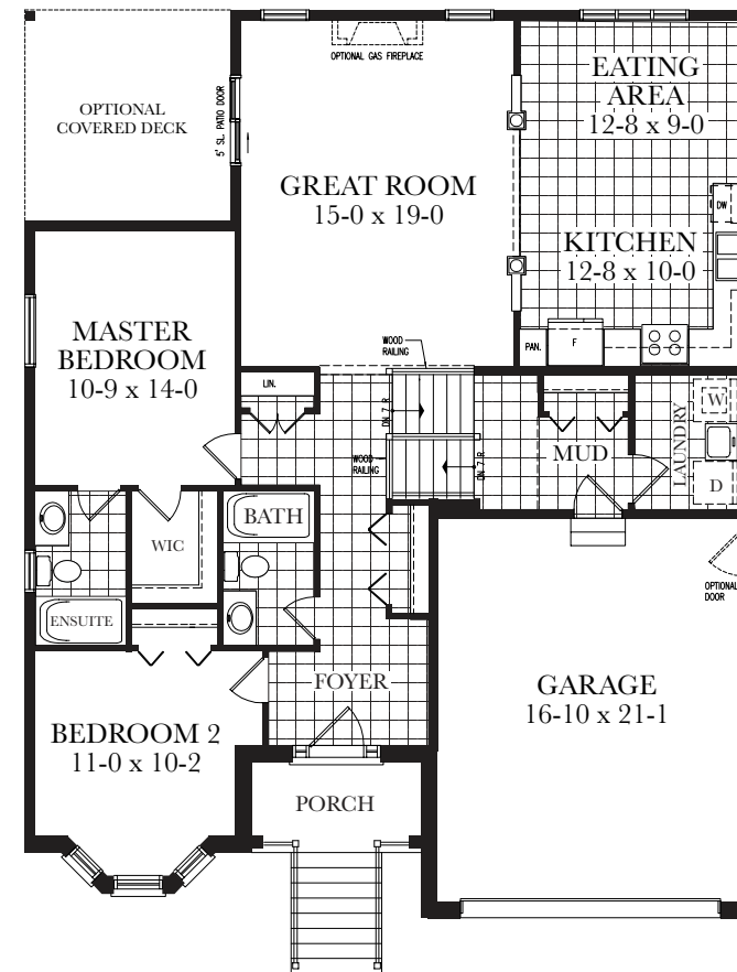
MAIN FLOOR PLAN ELEV. C - 1384 sq.ft
