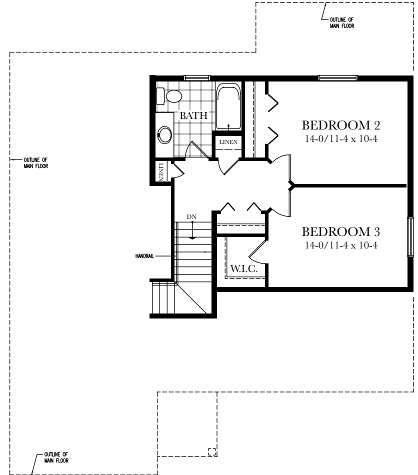
SECOND FLOOR PLAN - 573 sq.ft.
