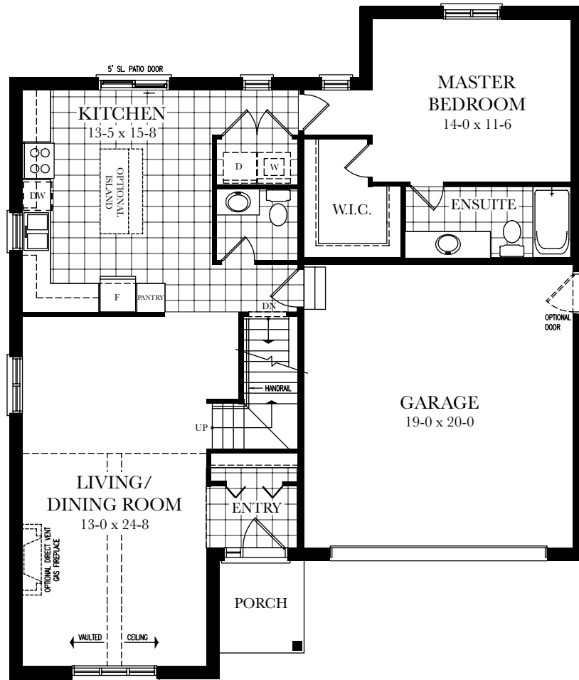
MAIN LEVEL PLAN - 1176 sq.ft.
