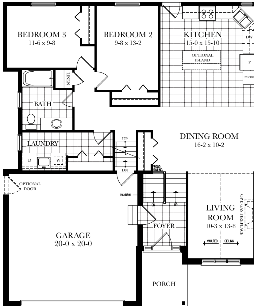
MAIN LEVEL PLAN - 1307 sq.ft.
