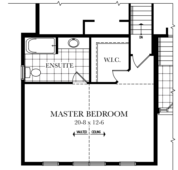
SECOND FLOOR PLAN - 479 sq.ft.
