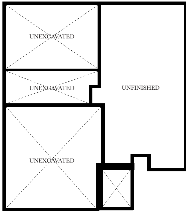
FOUNDATION PLAN
