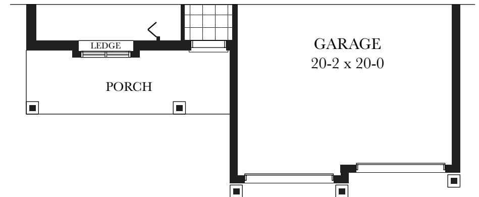
MAIN FLOOR PLAN ELEV. B - 1249 sq.ft.
