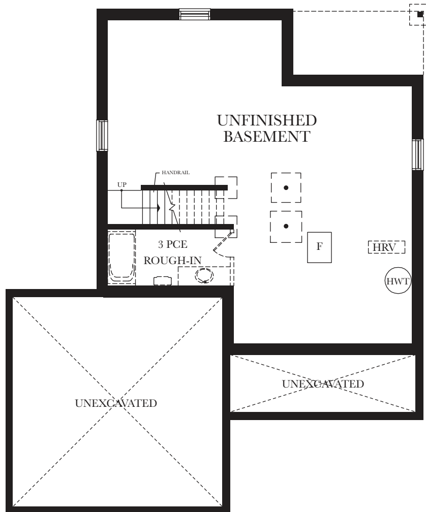
BASEMENT PLAN
