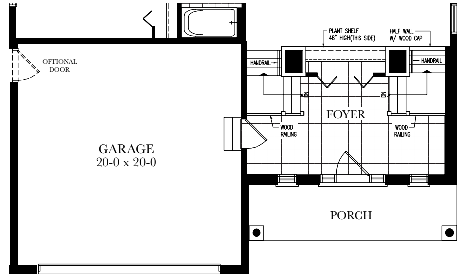
MAIN FLOOR PLAN ELEV. B - 1362 SQ.FT
