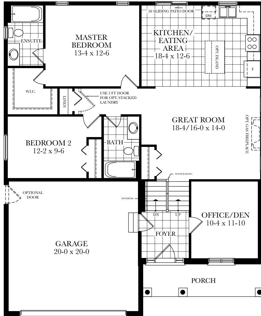
MAIN FLOOR PLAN ELEV. A - 1362 SQ.FT
