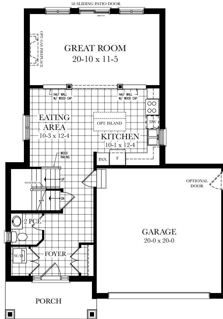
MAIN FLOOR PLAN ELEV. A 851 SQ.FT
