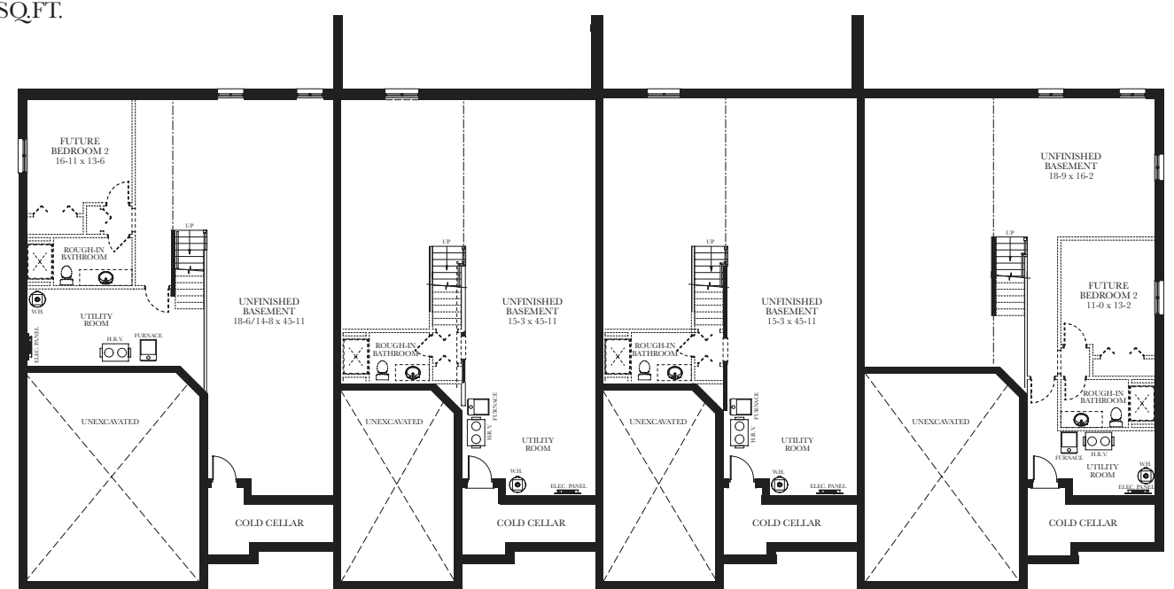
THE WATERLOO BASEMENT PLAN
